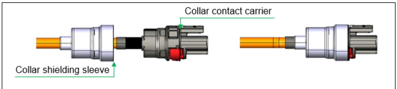
Figure 3.32: Representation 4.0 mm² SCC end position shielding sleeve on contact carrier (3.9 Slide the shielding sleeve onto the contact carrier)
