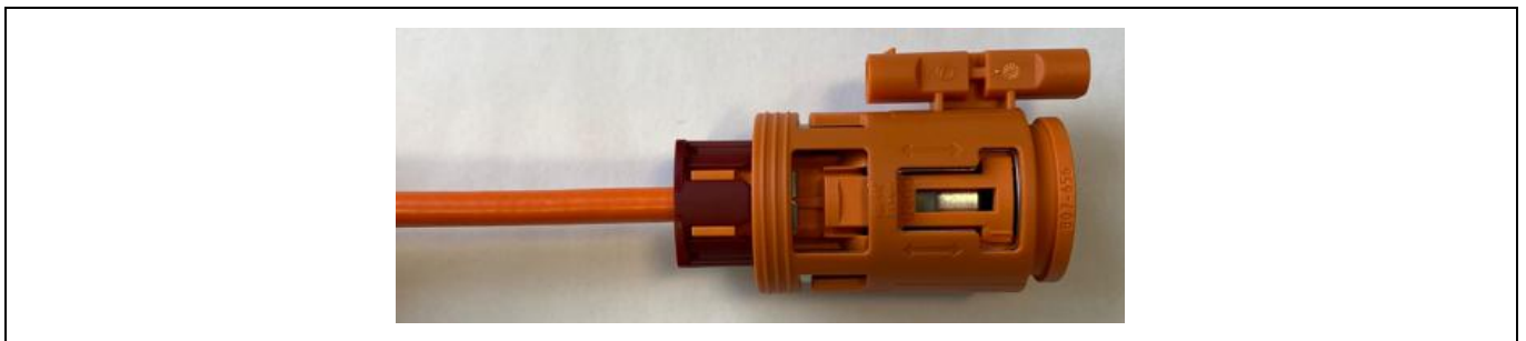
Figure 6.1: Representation 4.0 mm 2 & 6.0 mm 2 SCC assemble the In-Line CPA cover onto locking sleeve (6.1 Assemble the In-Line CPA cover)
