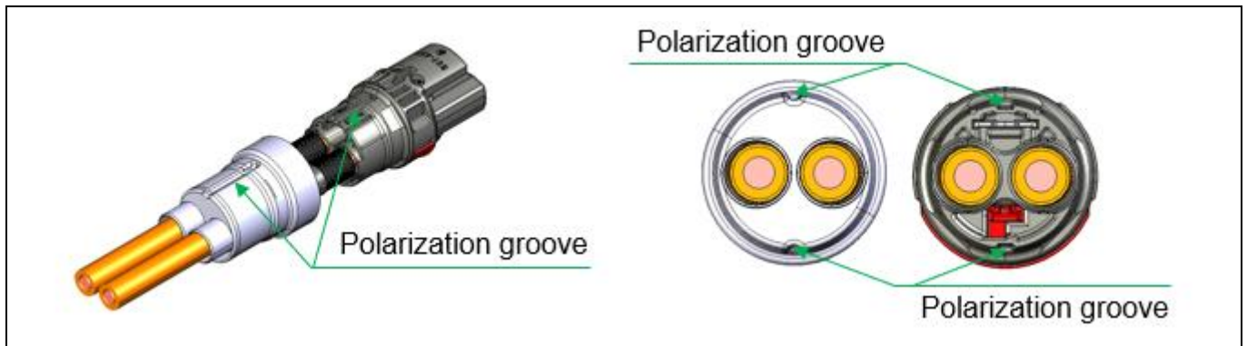
Figure 3.32: Representation 4.0 mm² SCC end position shielding sleeve on contact carrier (3.9 Slide the shielding sleeve onto the contact carrier)
