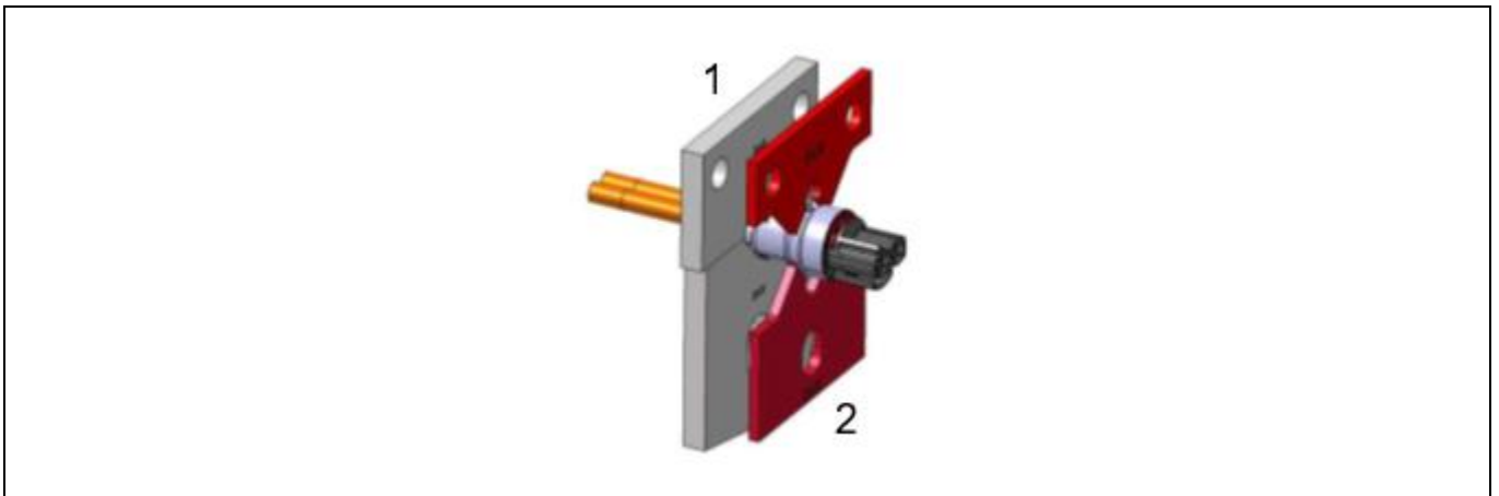
Figure 3.36: Representation 4.0 mm 2 SCC shielding crimping and contact carrier crimping (3.10 Crimp the shielding sleeve)
