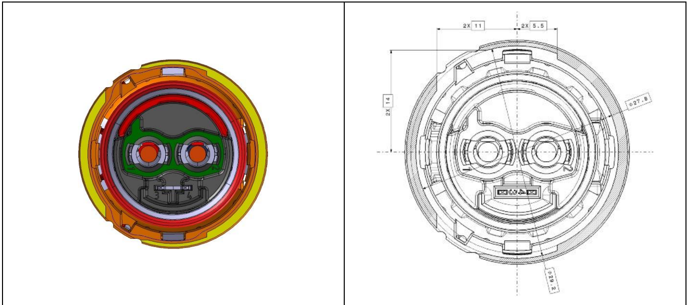
Figure 5.5: Representation 4.0 mm 2 & 6.0 mm 2 SCC dimension D\text{Ø}1 (5.1 Assembling the locking sleeve)
